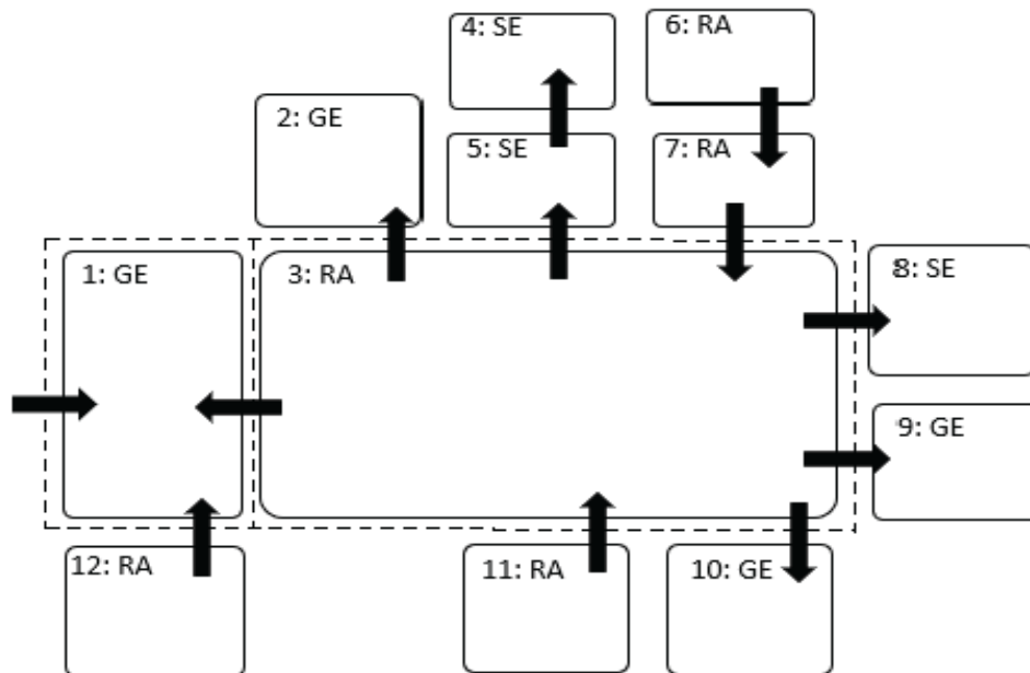
EMERGENCY CARE UNIT AIR FLOW RELATIONSHIPS
