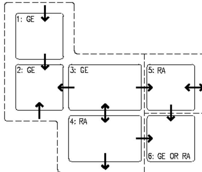
CENTRAL LAUNDRY FACILITY AIR FLOW RELATIONSHIPS
