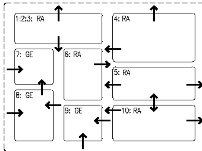
DENTAL CLINIC AIR FLOW RELATIONSHIPS
